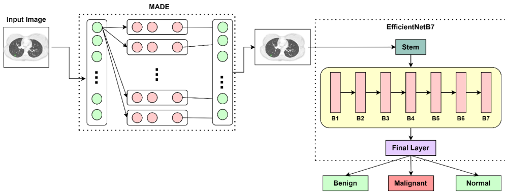
Figure 9. Proposed Mask-EffNet Model Architecture
