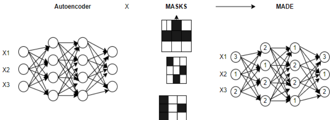
Figure 6. Architecture of MADE
