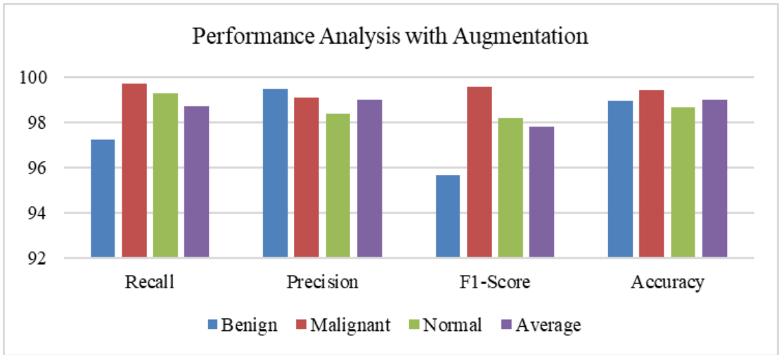
Figure 12. Performance analysis of the Mask-EffNet with Augmentation of dataset
