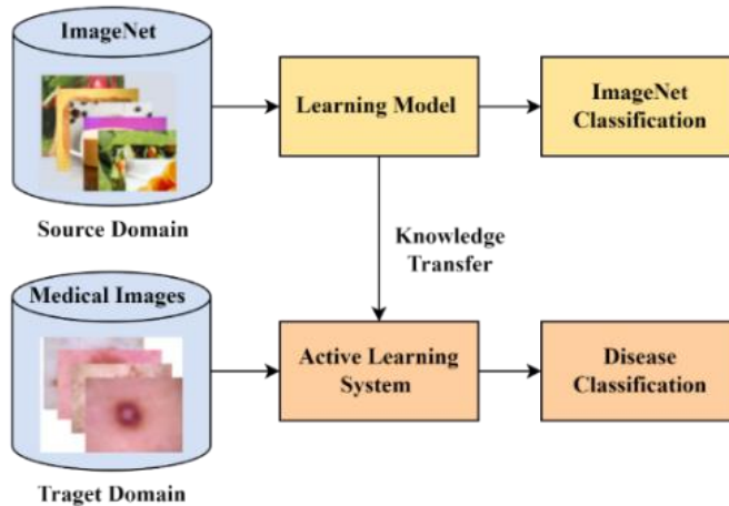
Figure 5. Architecture of Transfer Learning
