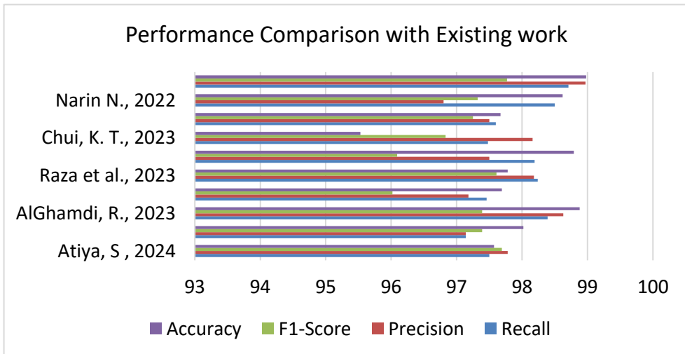
Figure 14. Performance Analysis comparison of the Mask-EffNet with different existing work
