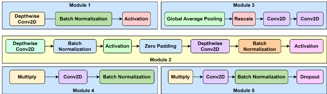
Figure 8. Modules in EfficientNetB7
