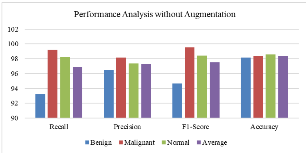
Figure 10. Performance analysis of the Mask-EffNet without Augmentation of dataset
