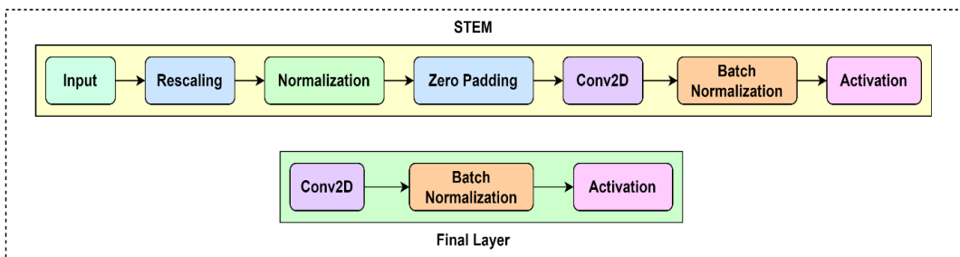
Figure 7. Stem and final layers of EfficientNetB7
