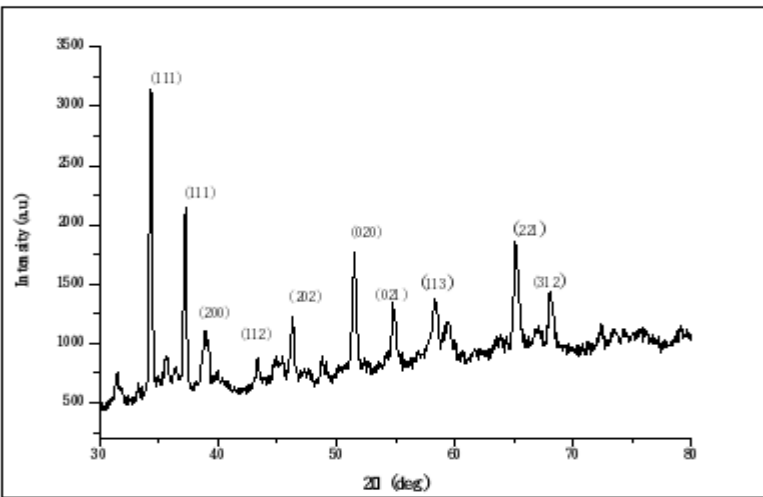
Figure 3: X-ray diffraction pattern of copper oxide nanoparticles
