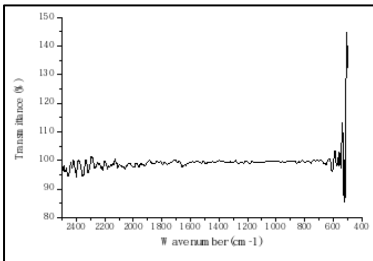
Figure 2: FTIR spectroscopy of copper oxide nanoparticles
