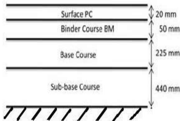
Fig. 6(a) Pavement structure on virgin soil for 2 msa
