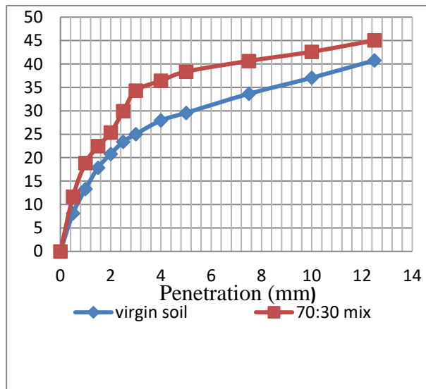
Fig 5: Effect of ceramic powder on the strength of soil
