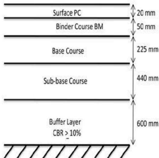
Fig. 6(a) Pavement structure on virgin soil for 2 msa
