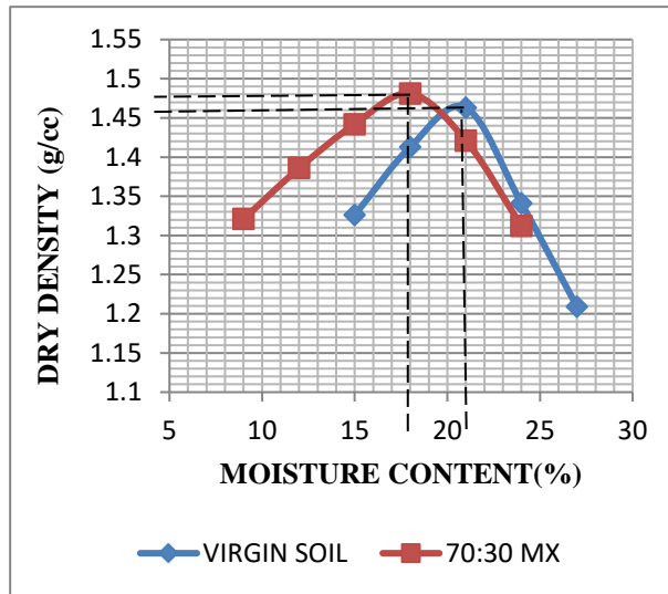
Fig 4: Effect of ceramic powder on the OMC and dry density of soil
