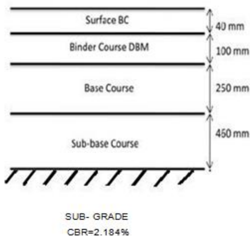
Fig. 7(b) Pavement structure on 70:30 mix for 10 msa.
