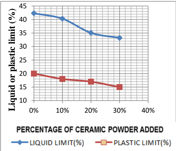
Fig. 2: Effect of ceramic powder on Atterberg’s limits of expansive soil
