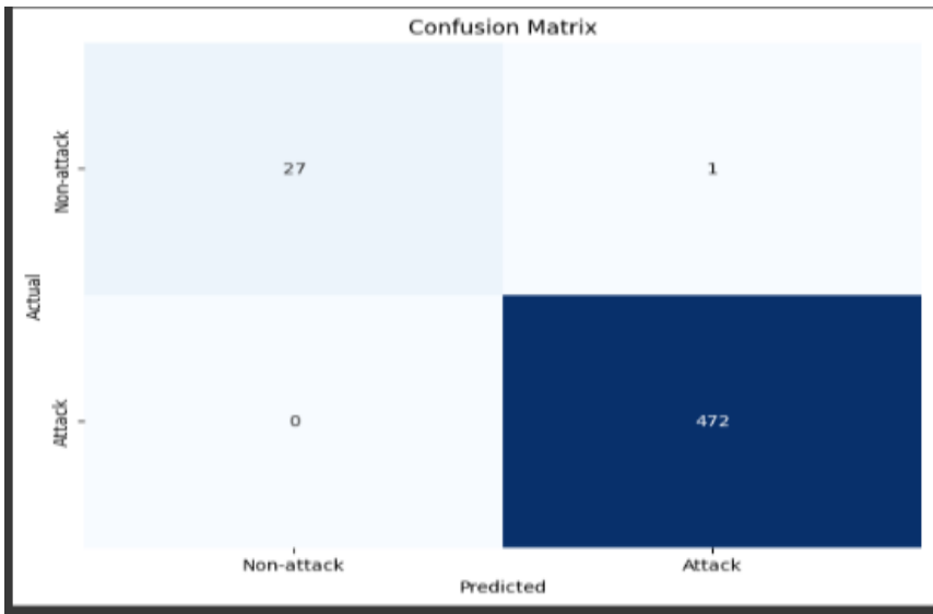
Figure 7. The confusion matrix shows the FN, TP, TN, and FP ratio on the BoT-IoT dataset of the hybrid model.
