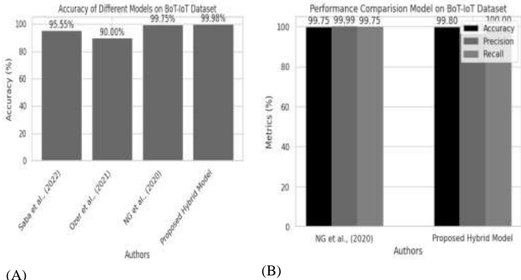
Figure 9. Comparison of the proposed hybrid machine learning model with previous studies.
