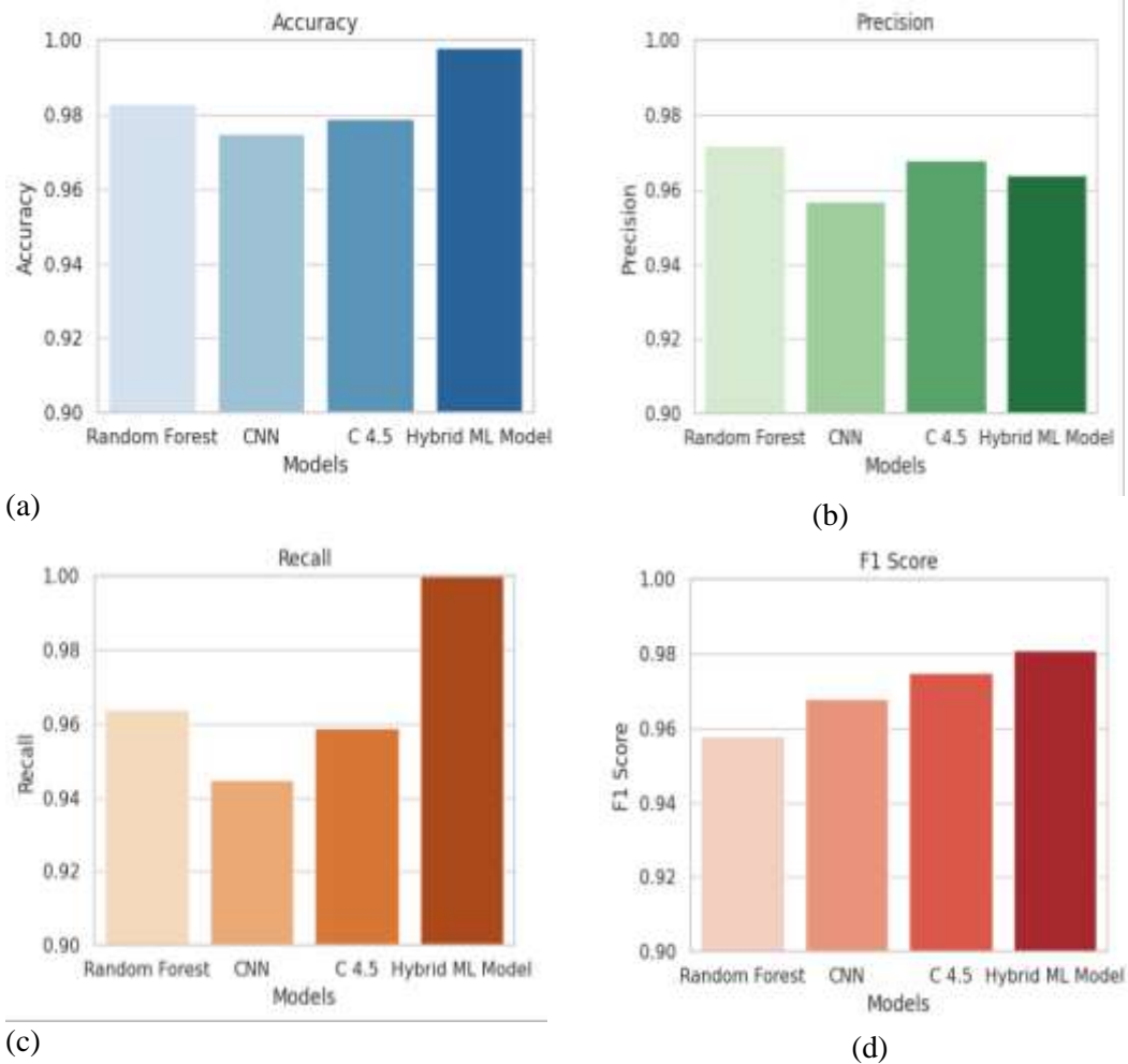
Figure 8. Comparison of the proposed hybrid model with CNN, Random Forest and C 4.5.
