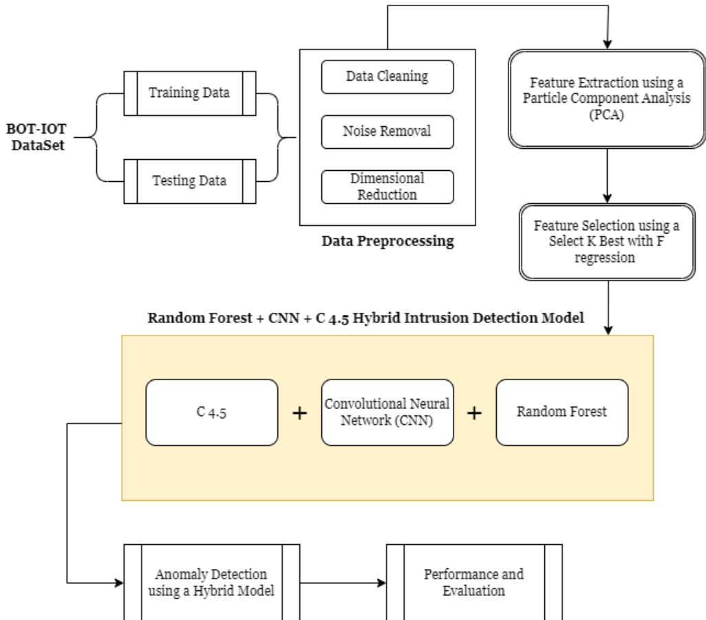
Figure 6. The proposed architecture of the suggested hybrid machine learning model is based on CNN, C 4.5, and Random Forest.
