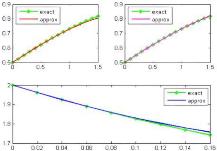
Figure 2: The comparison of logistic function(exact) as well approximation of the function(approximate) obtained by Mahgoub transform. The top two plots are shown for n=3 , n=5 at initial condition U_0=1/2 . The bottom plot for the initial condition U_0=2 .
