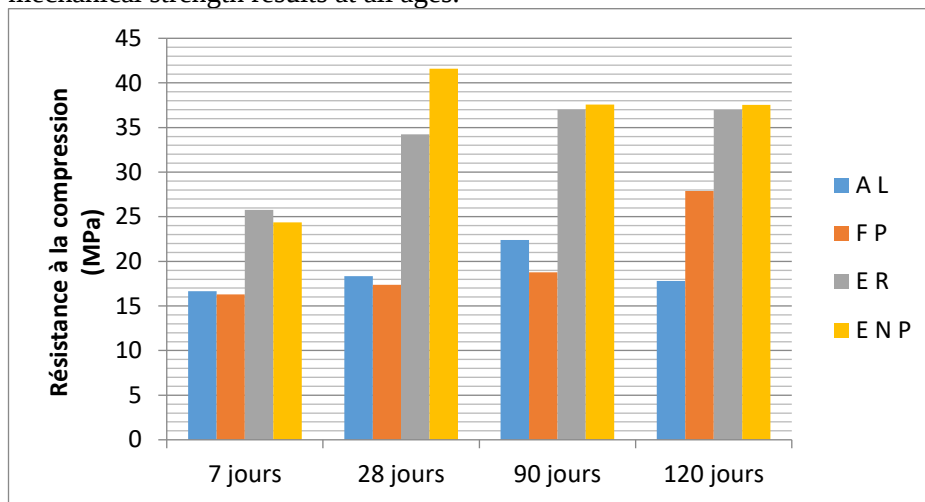
Figure 14. Compressive strength of sand concrete specimens with 10% SDP and 2 CNT at different media.
