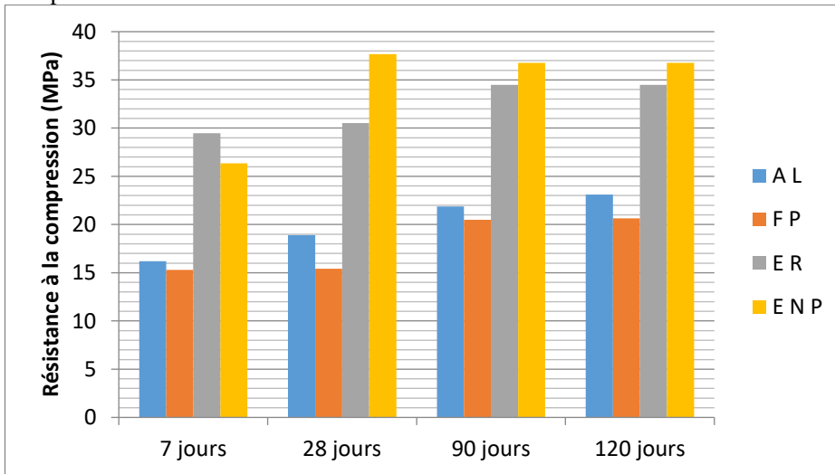
Figure 13. Compressive strength of sand concrete specimens with 5% SDP and 2% CNT at different media.
