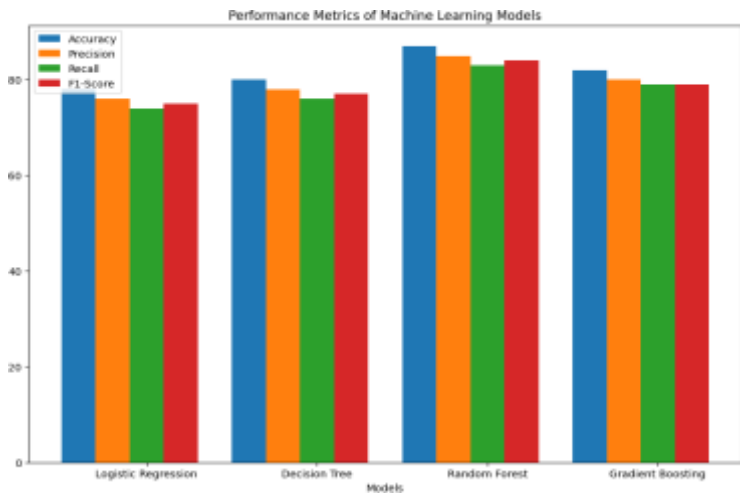
Figure 6 provides a bar graph comparing the performance metrics of different machine learning models. The Random Forest model shows superior performance with:
