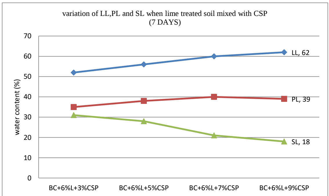
Fig. 6 Variation in Atterberg limits of BC soil – 6% lime mixture treated with various dosages CSP for 7-day testing
