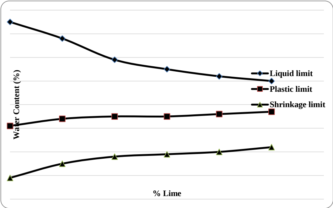
Fig. 2 Variation in Atterberg limits of BC soil treated with various dosages of lime for immediate testing
