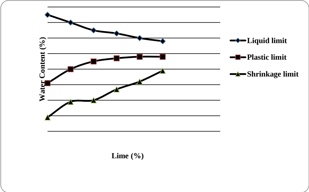
Fig. 3 Variation in Atterberg limits of BC soil treated with different dosages of lime for 7-day curing
