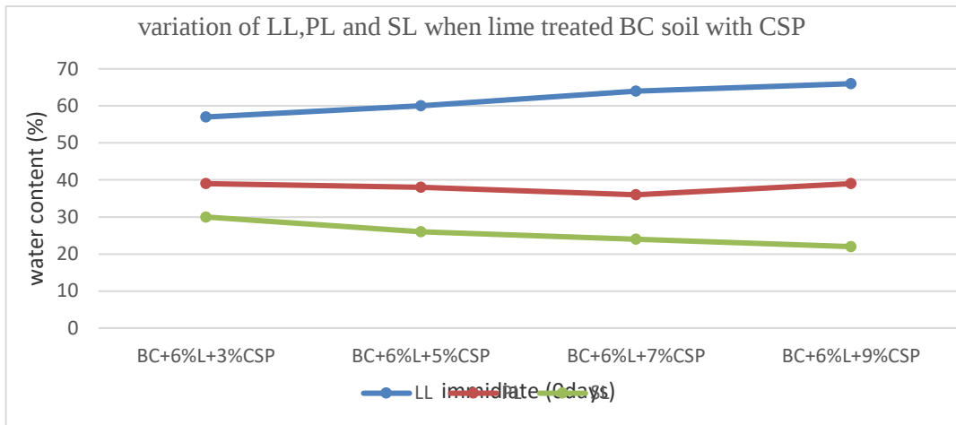
Fig. 5 Variation in Atterberg limits of BC soil – 6% lime mixture treated with various dosages of CSP for immediate testing
