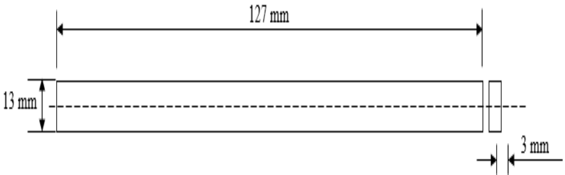
Figure. 3 Detail Drawing of Flexural Test Specimen as per ASTM D790
