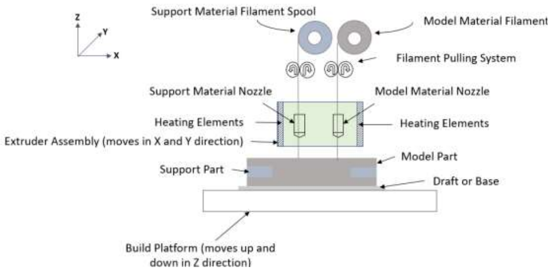
Figure. 1 Schematic diagram of Fused Deposition Modeling (FDM) Process
