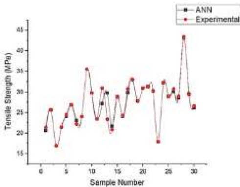
Figure. 7 Statistical stability and relationship in proposed ANN for (a) Tensile Strength (b) Flexural Strength
