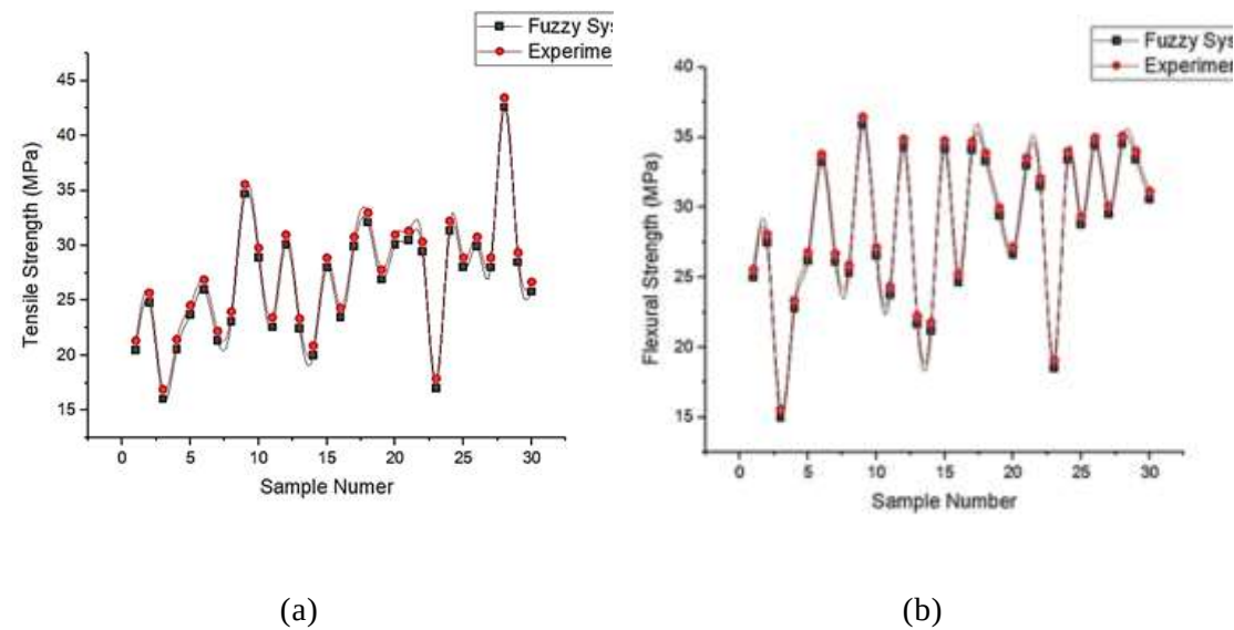
Figure. 6 Comparison between Fuzzy System and Experimental obtained (a) Tensile strength (b) Flexural Strength
