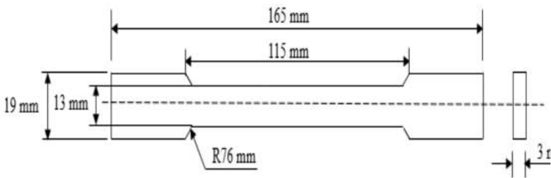
Figure. 2 Detail Drawing of Tensile Test Specimen as per ASTM D638 type-I
