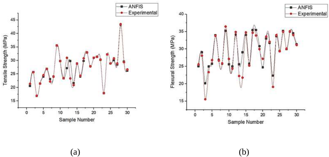
Figure. 9 Comparison between ANFIS and Experimental obtained (a) Tensile strength (b) Flexural Strength
