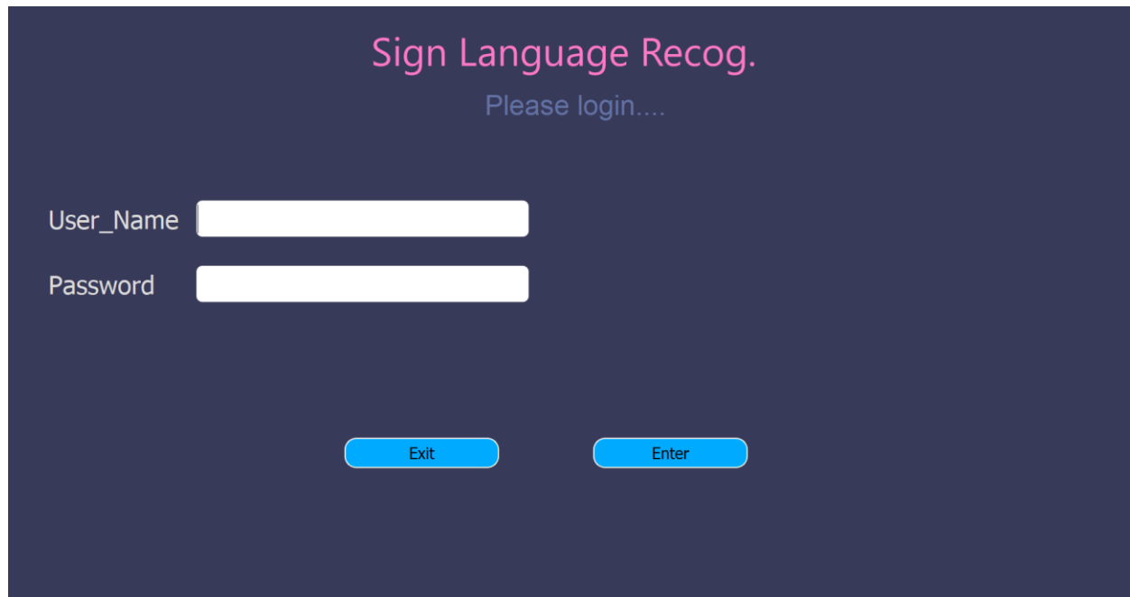
Figure 1 App GUI
