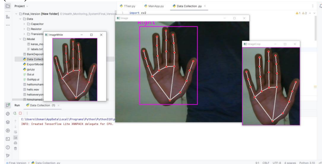
Figure 2 Dataset Creation
