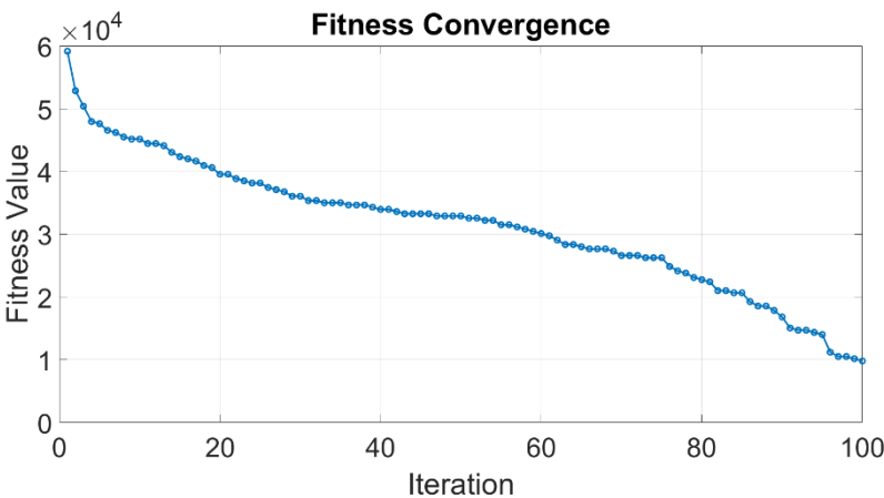
Figure No 4: Convergence graph for IEEE 57 bus at multi-objective function
