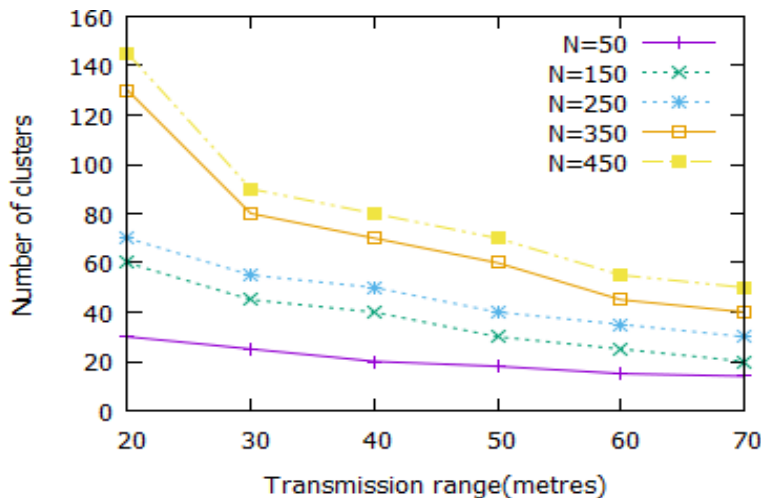
Figure 4: Transmission range against number of clusters
