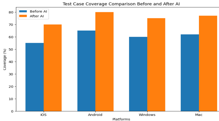
Figure 5 displays a bar chart comparing test case coverage before and after AI adaptation. The AI model improved test case coverage from an average of 60% to 75% across different platforms.
