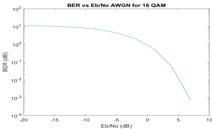
Figure 9: BER Value
